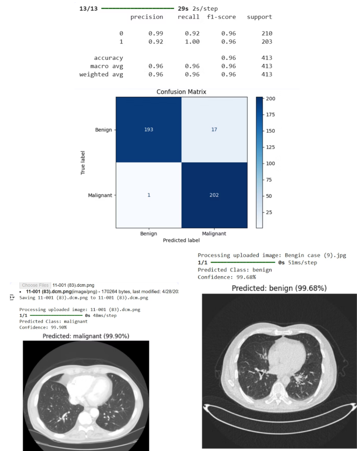
Figure 1: MobileNetV2 model visualizations and outputs.
