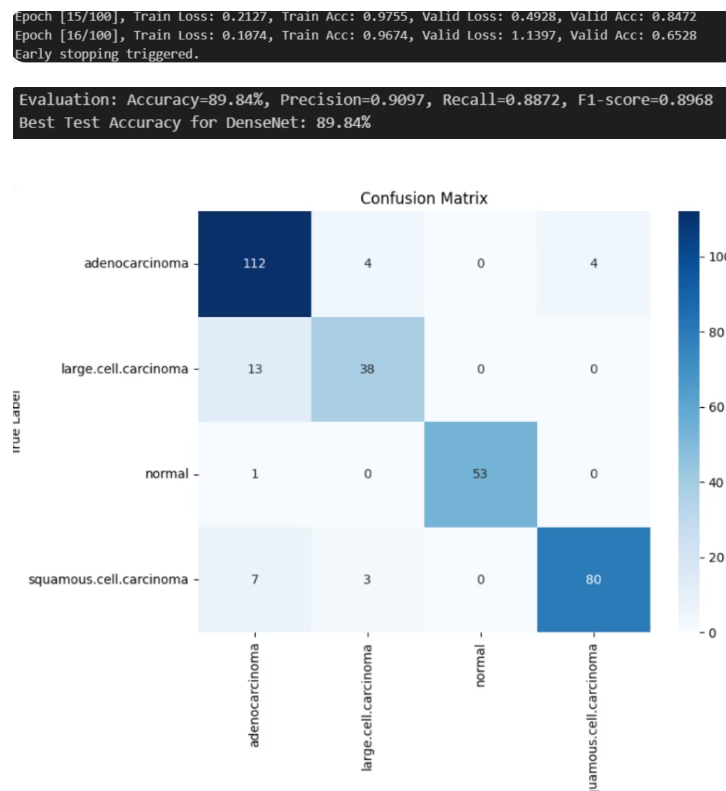
Figure 4: DenseNet121 model visualizations and outputs.
